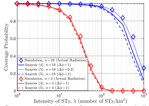
Fig. 2: Coverage probability of spectrum-shared directional wireless network with ULA antenna.
