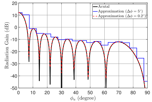
Fig. 1: Actual and approximated radiation gain of ULA.
